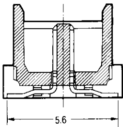
Section X-X
