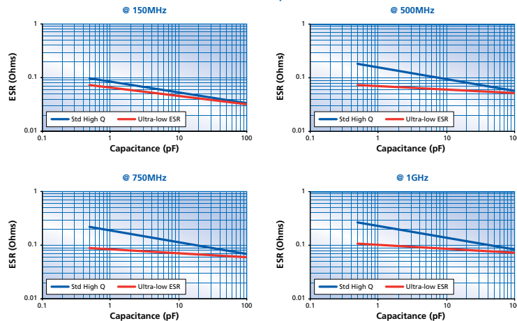
ESR vs. Capacitance
