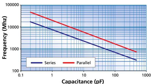
Resonant Frequency vs Capacitance 0805 case size
