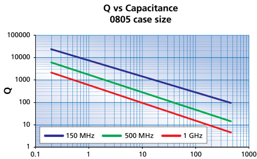
Q vs Capacitance 0805 case size
