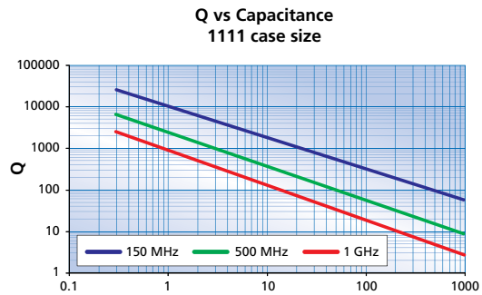
Q vs Capacitance 1111 case size
