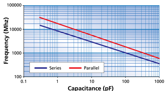
Resonant Frequency vs Capacitance 1111 case size
