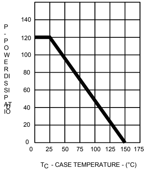
Figure 1. Power Derating
