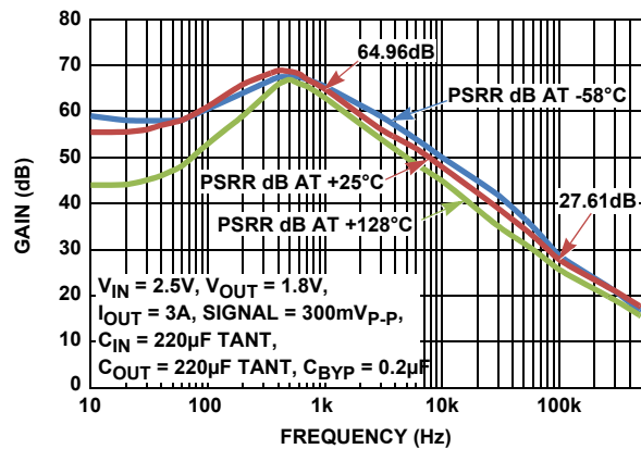
FIGURE 28. PSRR
