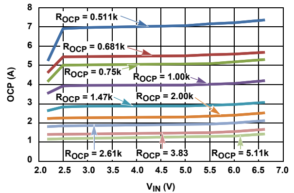
FIGURE 18. R_{OCP} vs OCP AT +25 °C, V_{OUT} = 1.5V
