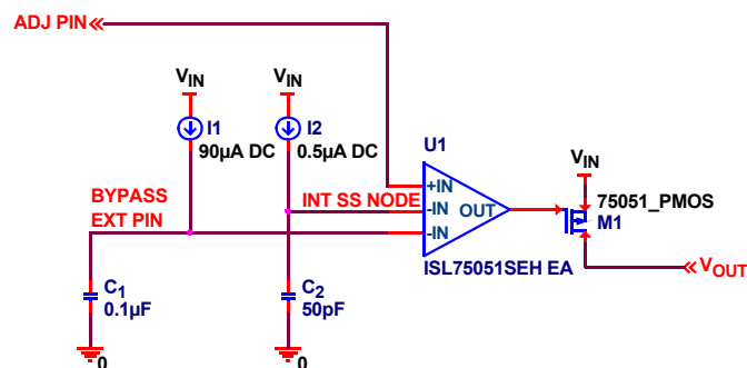
FIGURE 31. SOFT-START
