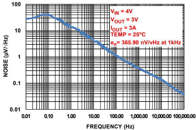
FIGURE 27. NOISE (µV/√Hz)
