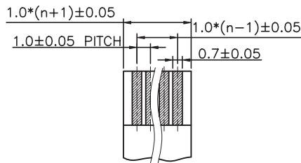
APPLICABLE FFC LAYOUT 5 (THICKNESS: FROM 0.29 MM to 0.34 MM)
