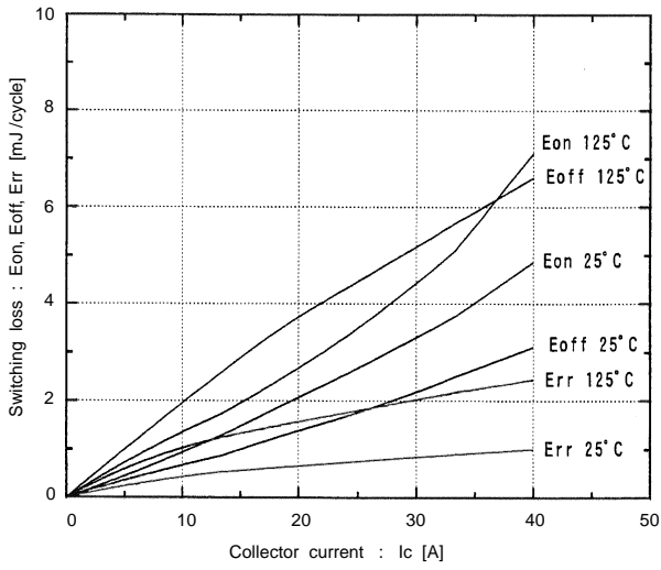
Switching loss vs. Collector current V_{cc}=600V, R_G=51\text{ ohm}, V_{GE}=\pm 15V
