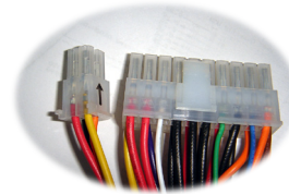
20+4 pin ATX power connector
