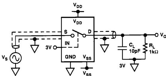
TEST CIRCUIT 5 OFF ISOLATION
