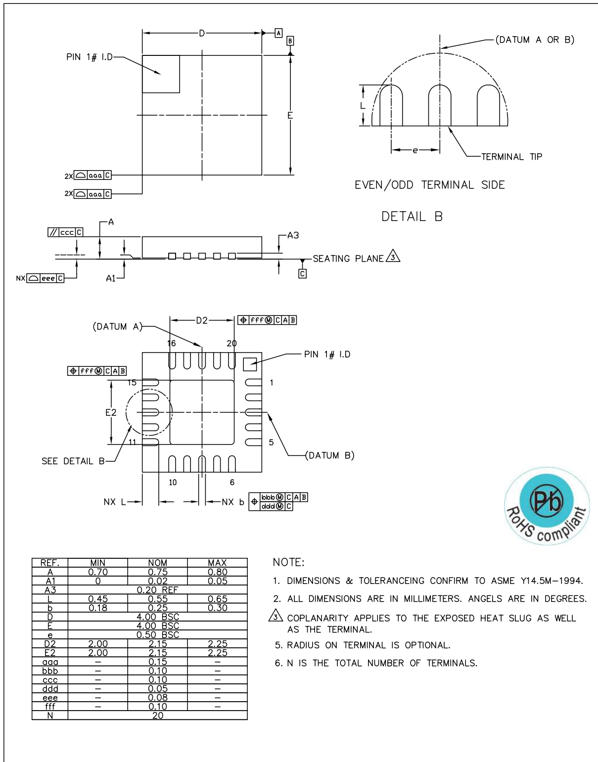
Figure 37. QFN(4x4)-20 Package
