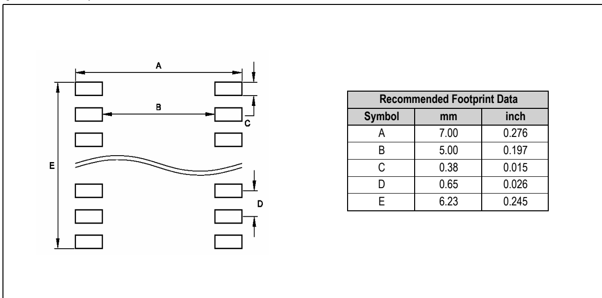
Figure 18. PCB Footprint
