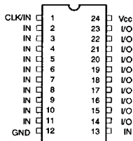
DIP/SOIC
