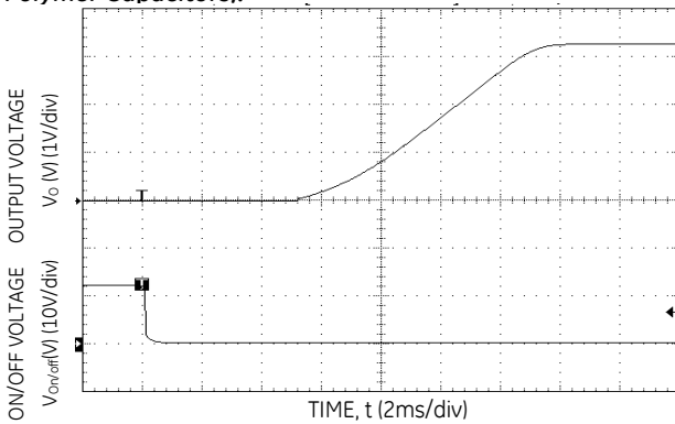
Figure 14. Typical Start-Up Using Remote On/Off ( V_{in} = 12.0Vdc , V_o = 3.3Vdc , I_o = 3A ).
