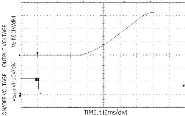
Figure 15. Typical Start-Up Using Remote On/Off with Low-ESR external capacitors (7x150uF Polymer) ( V_{in} = 12.0Vdc , V_o = 3.3Vdc , I_o = 3A , C_o = 1050\mu F ).
