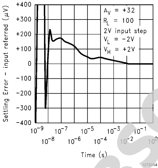
Settling, Unclamped
