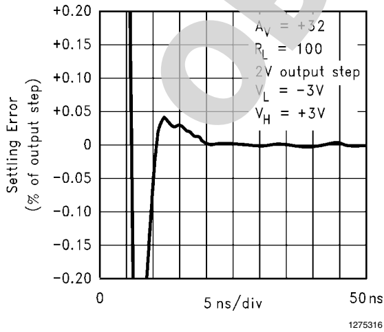
Settling, Unclamped
