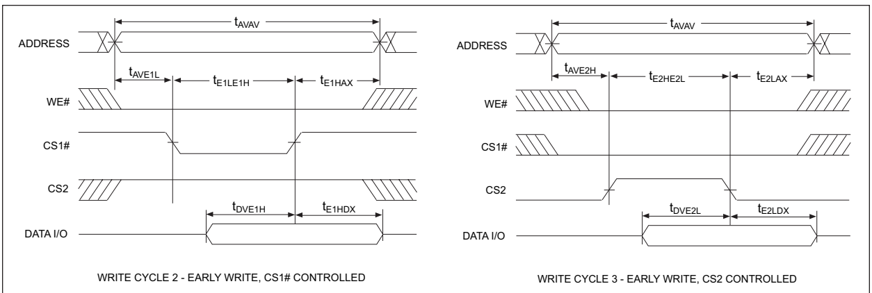
FIGURE 4 – WRITE CYCLES 2
