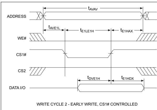
FIGURE 4 – WRITE CYCLES 2
