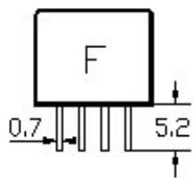
TIN/LEAD PLATED PINS
