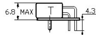
TIN PLATED RIGHT ANGLE PINS WITH REMOVABLE ISOLATING PADS
