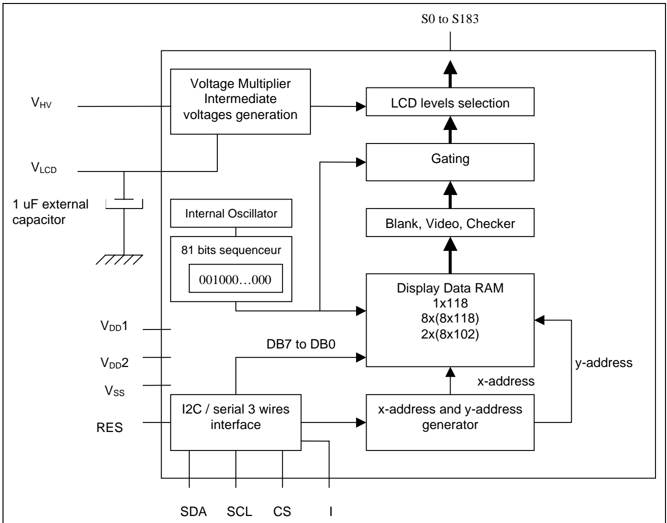
Figure 9: Block diagram.
