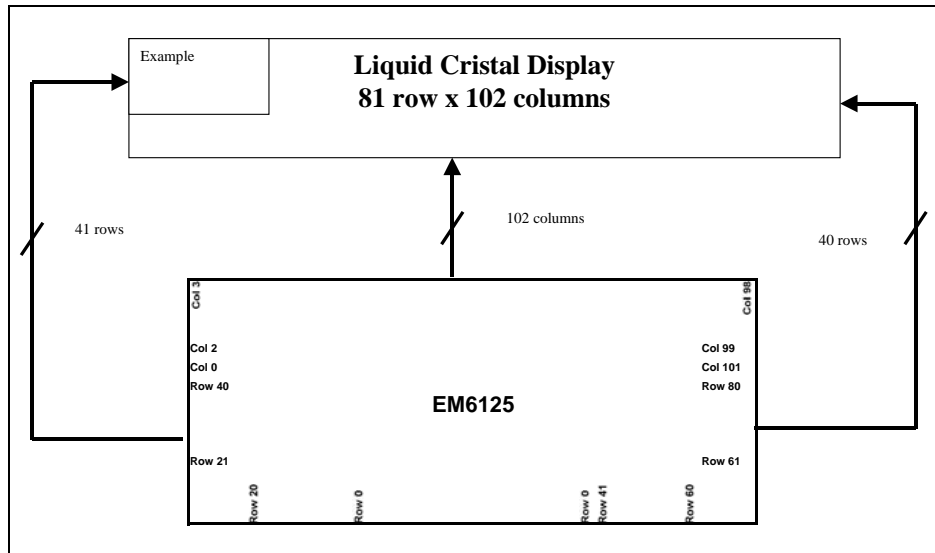
Figure 38: Connection between EM6125 and LCD for the application example
