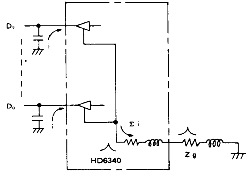
Figure 11 Cause of the Noise
