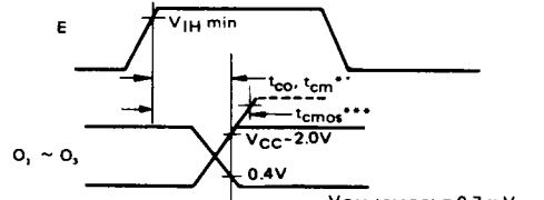
Figure 6 Output Delay
