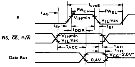
Figure 1 Bus Read Timing (Read Information from PTM)
