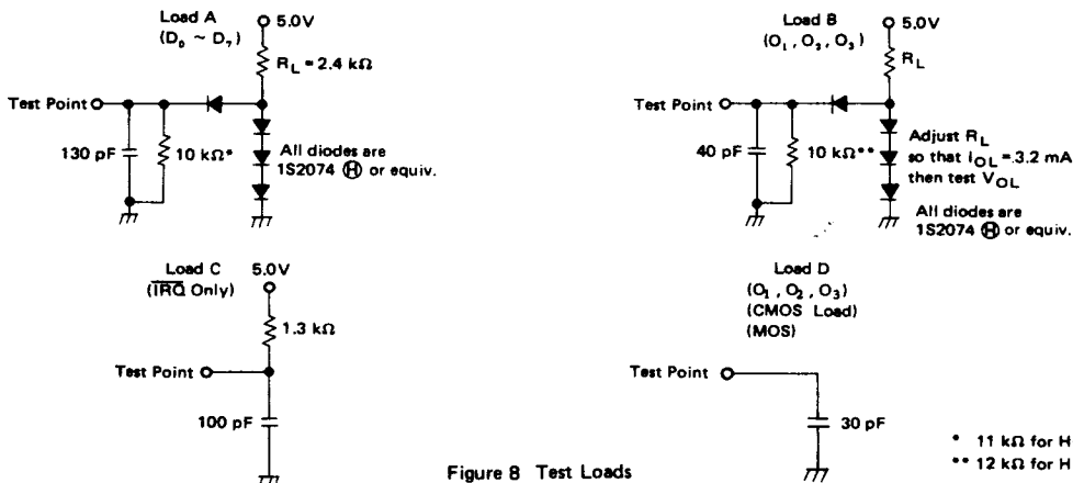
Figure 8 Test Loads
