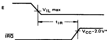
Figure 7 \overline{IRQ} Release Time
