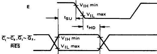
Figure 5 Input Setup and Hold Times
