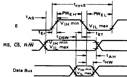
Figure 2 Bus Write Timing (Write Information into PTM)
