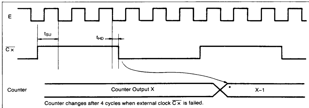
Figure A. External Clock Synchronous Timing
