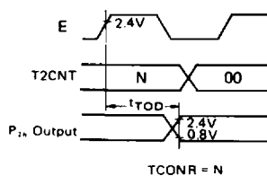
(b) Timer 2 Output Timing
