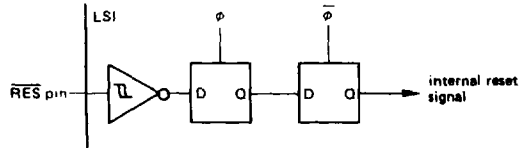
Figure 30 \overline{RES} circuit
