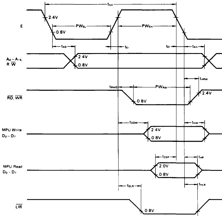
Figure 1 Bus Timing
