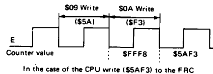
Figure 17 Counter Write Timing
