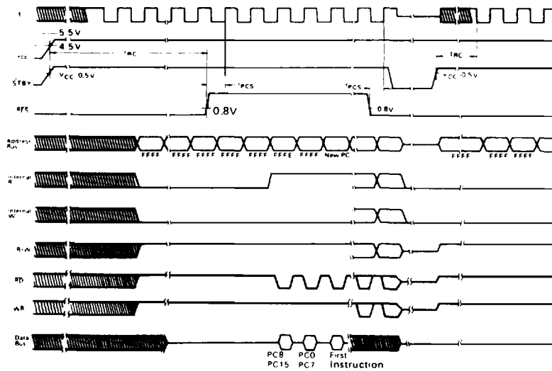
Figure 11 Reset Timing
