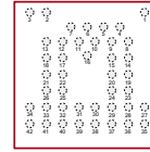
42-Ball Bumped Die (BD) (bottom view)
