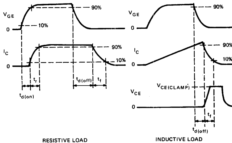
FIGURE 9. SWITCHING WAVEFORMS
