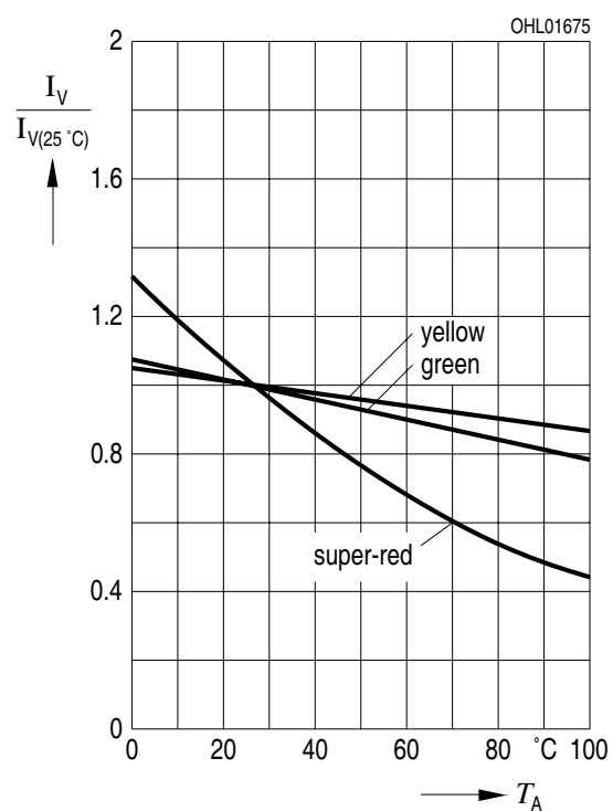
Relative Lichtstärke I_V/I_{V(25\text{ °C})} = f(T_A) Relative Luminous Intensity I_F = 10\text{ mA}
