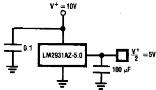
(b) Voltage Regulator
