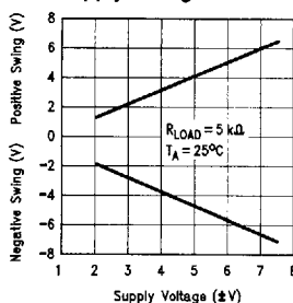
Output Swing vs Supply Voltage
