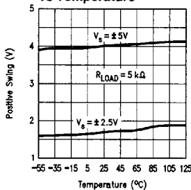
Positive Output Swing vs Temperature
