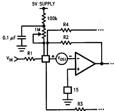
FIGURE 24. Method for Trimming V_{OS}
