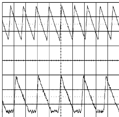
CCM and DCM Operating Modes V_{IN} = 24\text{V} , V_O = 3.3\text{V} , I_O = 3\text{A}/0.4\text{A} 2 \mu\text{sec/div}
