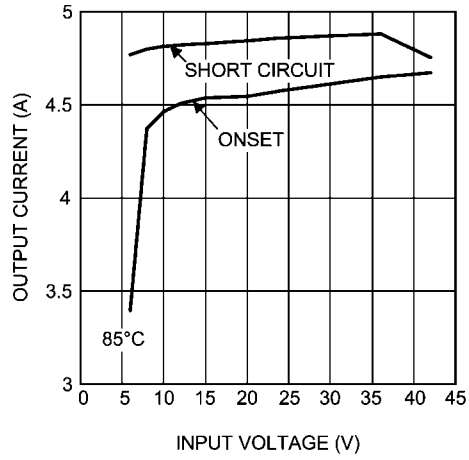
Current Limit 3.3V_{OUT} @ 85^\circ C
