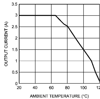
Thermal derating curve V_{IN} = 24V , V_{OUT} = 5.0V ,
