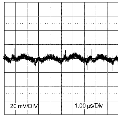
Output Ripple 24V IN 3.3V O 3A, BW = 200 MHz
