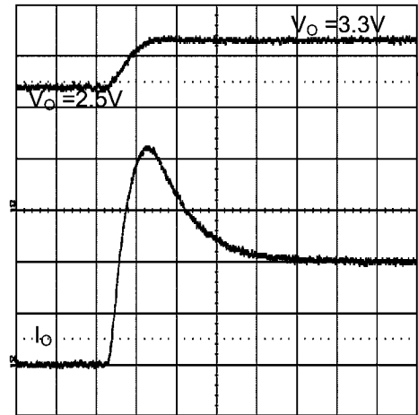
Pre-Biased Startup
