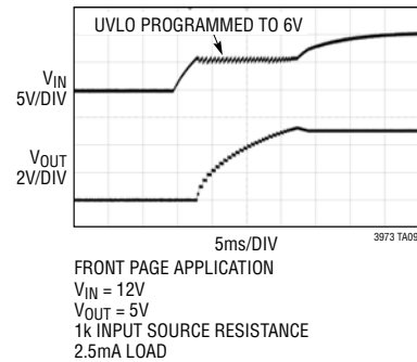
Start-Up from High Impedance Input Source
