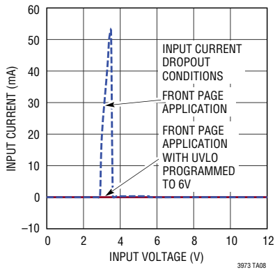
Input Current During Start-Up
