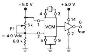
FIGURE 2 — CRYSTAL CONTROLLED MULTIVIBRATOR
