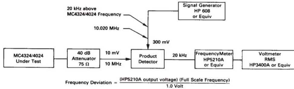
FIGURE 11 — NOISE DEVIATION TEST CIRCUIT
