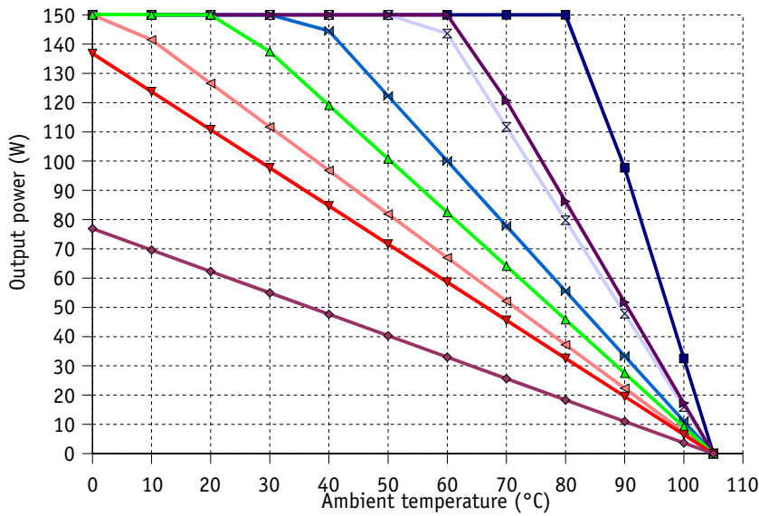
MGDS-150-O-x Series Thermal Curves
