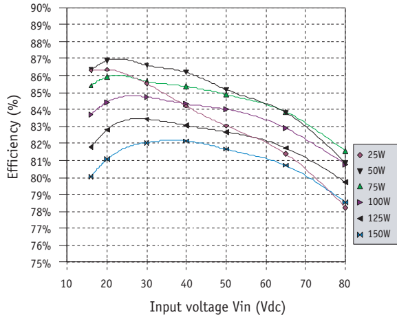
Typical efficiency MGDS-150-0-E at 25°C
