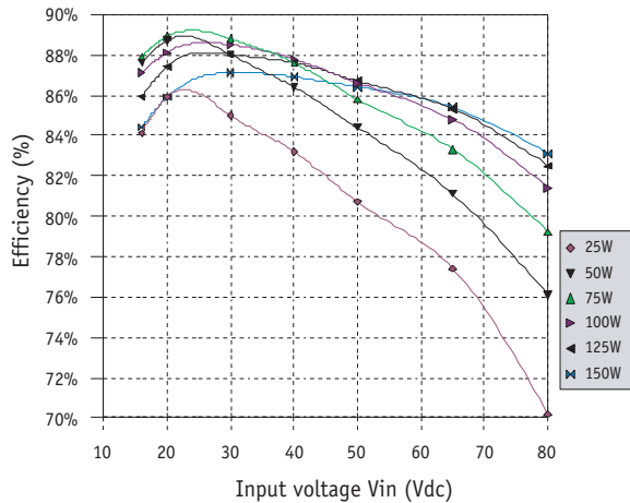
Typical efficiency MGDS-150-0-I at 25°C
