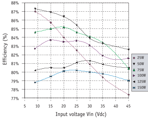
Typical efficiency MGDS-150-H-E at 25°C
