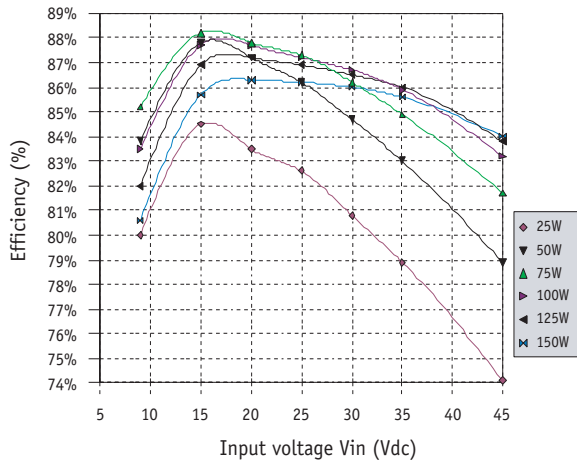
Typical efficiency MGDS-150-H-I at 25°C
