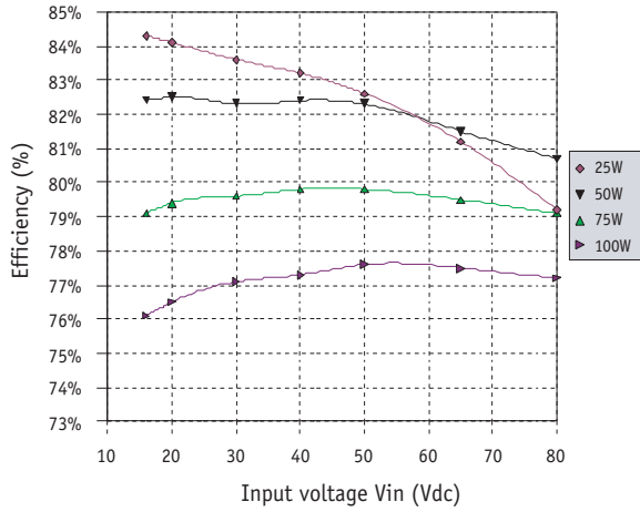
Typical efficiency MGDS-150-0-B at 25°C
