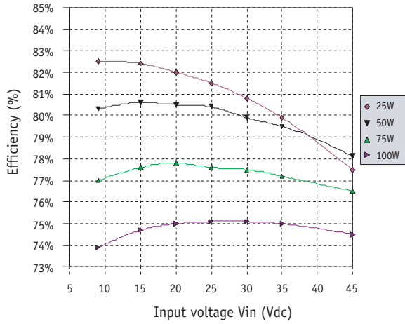
Typical efficiency MGDS-150-H-B at 25°C
