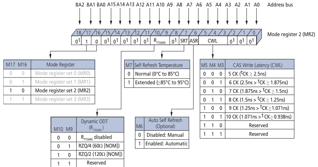
Figure 50: Mode Register 2 (MR2) Definition
