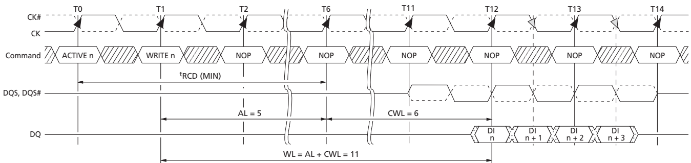
Figure 51: CAS Write Latency
