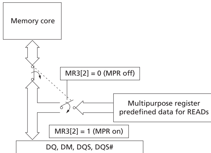
Figure 53: Multipurpose Register (MPR) Block Diagram
