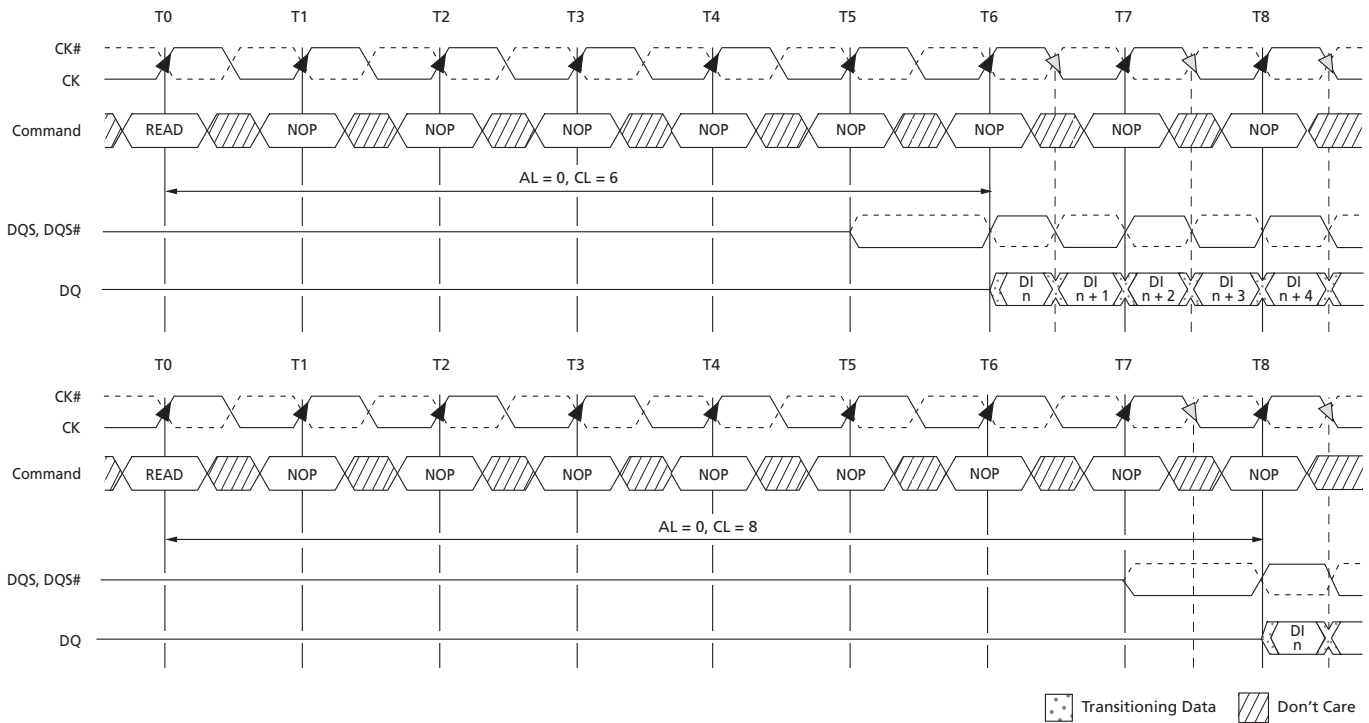
Figure 47: READ Latency
