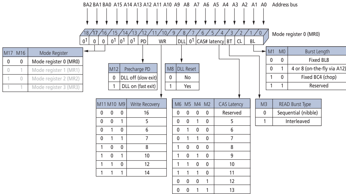
Figure 46: Mode Register 0 (MR0) Definitions
