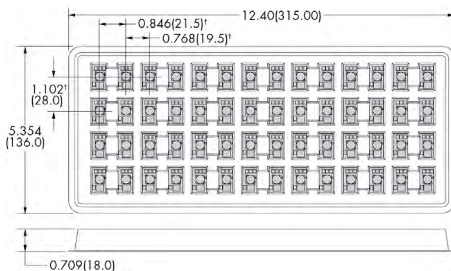
TRAY DIMENSIONS (TOP VIEW)
