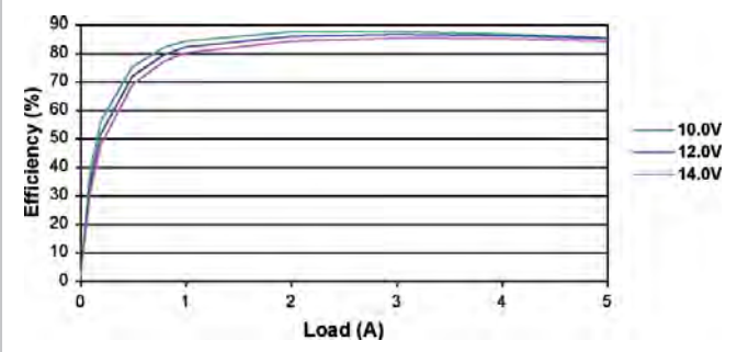
V OUT = 1.2V
