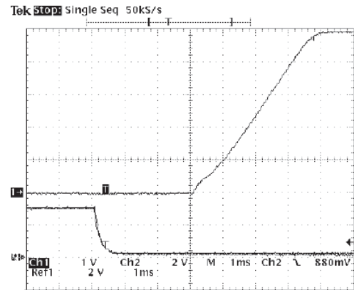
TYPICAL START-UP USING REMOTE ON/OFF
