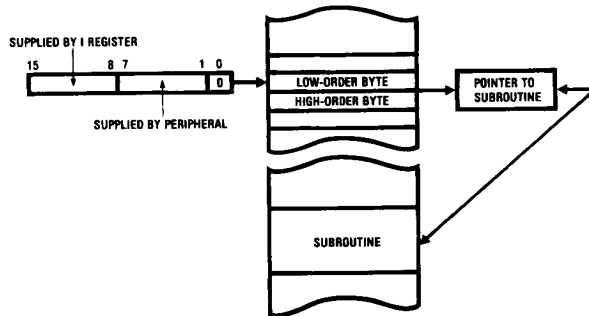
FIGURE 17. Interrupt Mode 2
