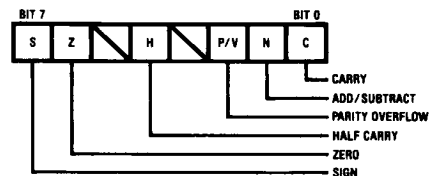
FIGURE 5. Flag Register
