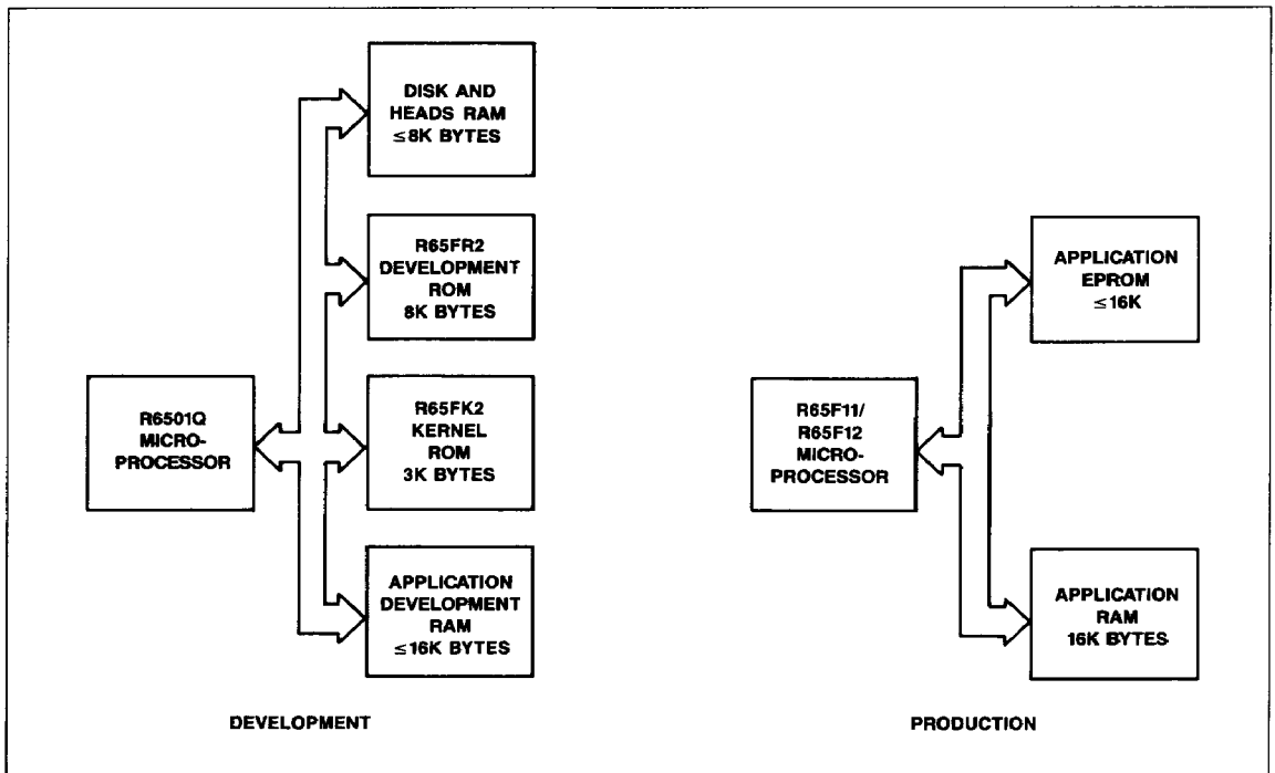
Figure 2. R65FR2 and R65FK2 Configuration 2 Block Diagrams
