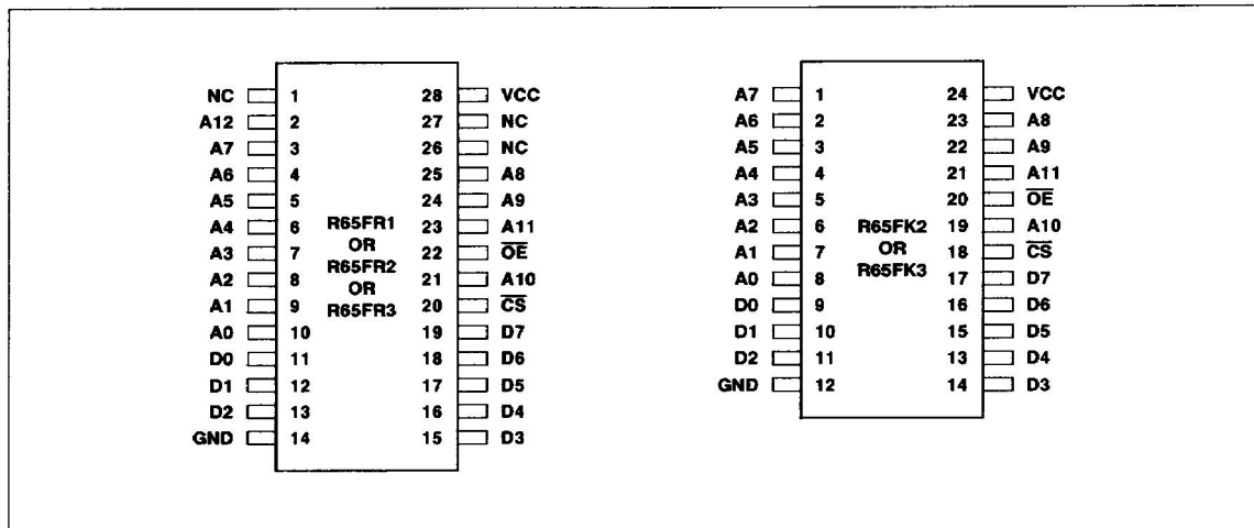
RSC-FORTH ROM Pin Assignments
