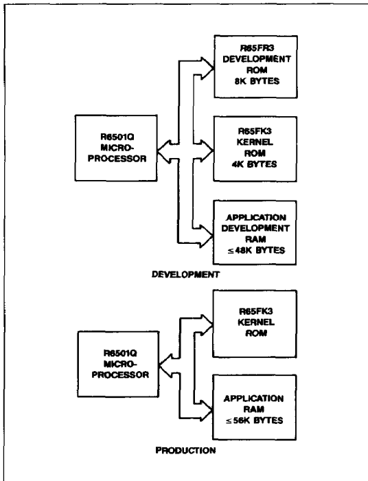
Figure 4. R65FR3 and R65FK3 Configuration 3 Block Diagrams
