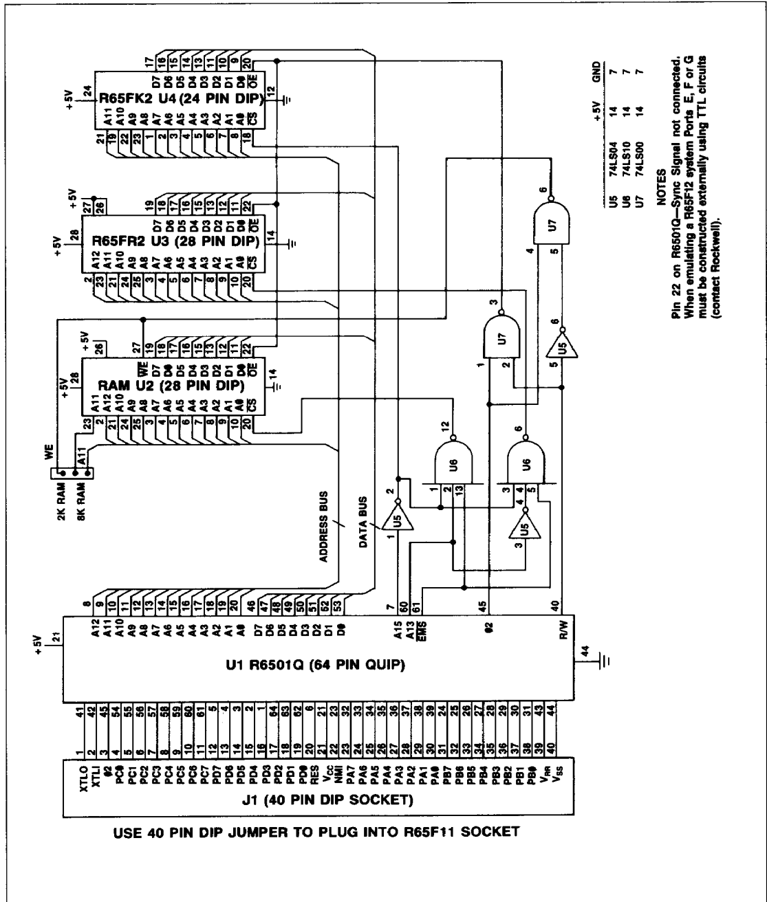
Figure 3. R6501Q, R65FR2 and R65K2 Application Configuration Schematic
