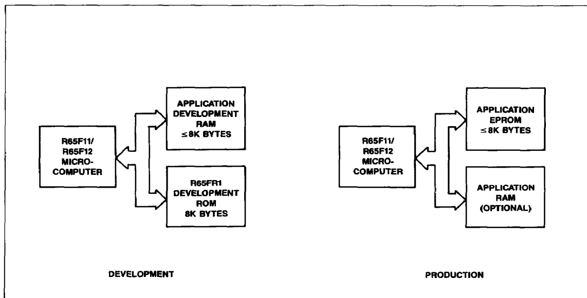
Figure 1. R65FR1 Configuration 1 Block Diagram
