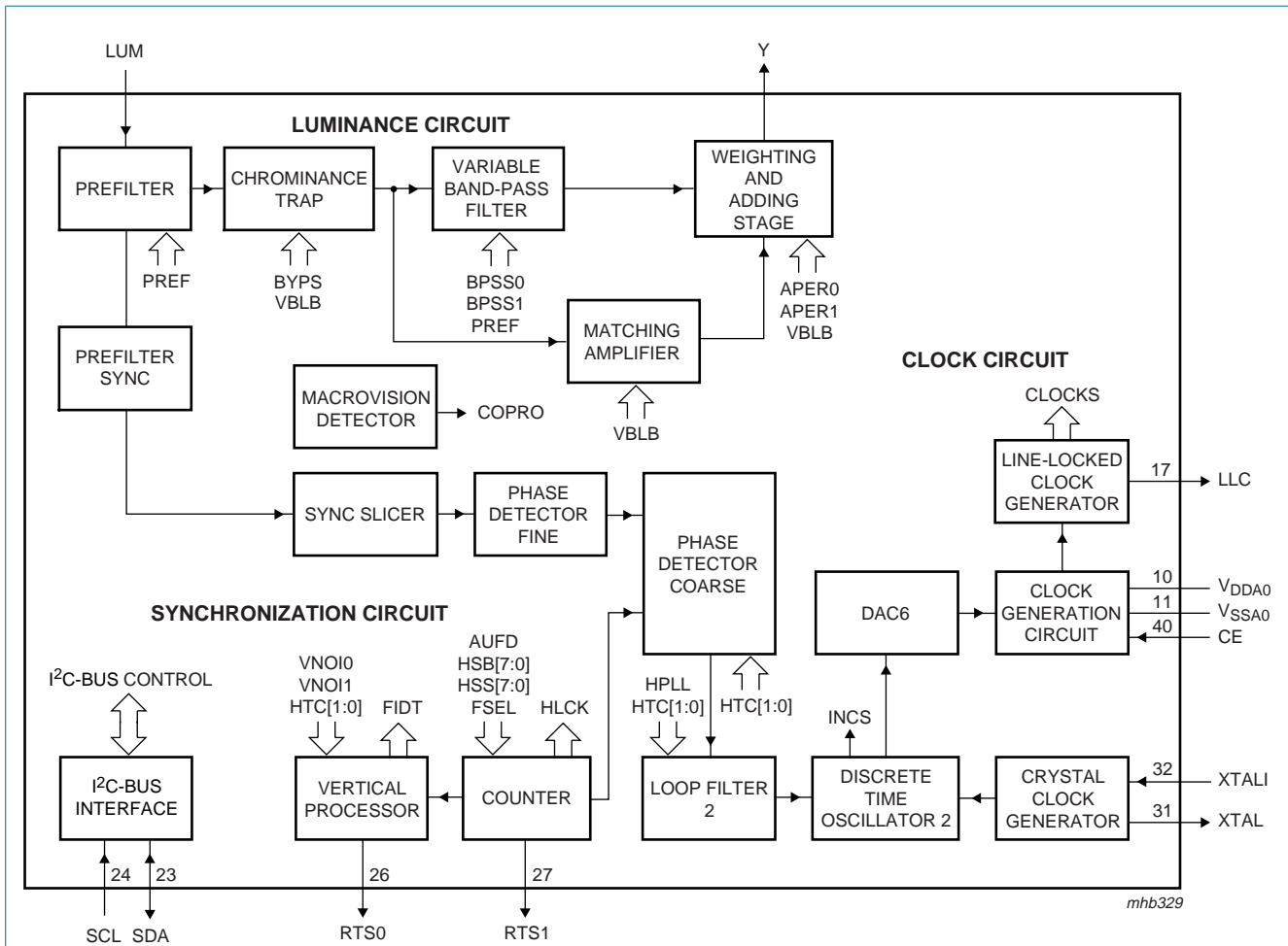
Fig 19. Luminance and sync processing
