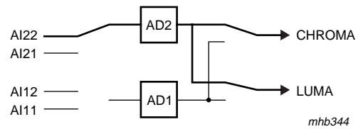
Fig 30. Mode 3; CVBS (automatic gain)
