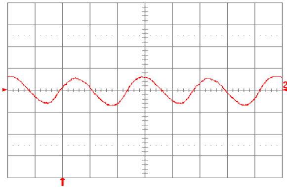
Fig. 6.0V.15: Input reflected ripple current, i_c (100 mA/div.), measured at input terminals at full rated load current and V_{in} = 24\text{V} . Refer to Fig. 6.0V.14 for test setup. Time scale: 1 \mu\text{s}/\text{div} .
