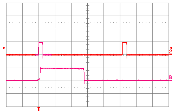
Fig. 1.5V.18: Load current (top trace, 20 A/div., 20 ms/div.) into a 10 \text{m}\Omega short circuit during restart, at V_{in} = 24\text{V} . Bottom trace (20 A/div., 2 ms/div.) is an expansion of the on-time portion of the top trace.
