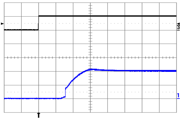
Fig. 1.0V.10: Turn-on transient at full rated load current (resistive) plus 10,000\mu\text{F} at V_{in} = 24\text{V} , triggered via ON/OFF pin. Top trace: ON/OFF signal (5 V/div.). Bottom trace: output voltage (0.5 V/div.). Time scale: 1 ms/div.
