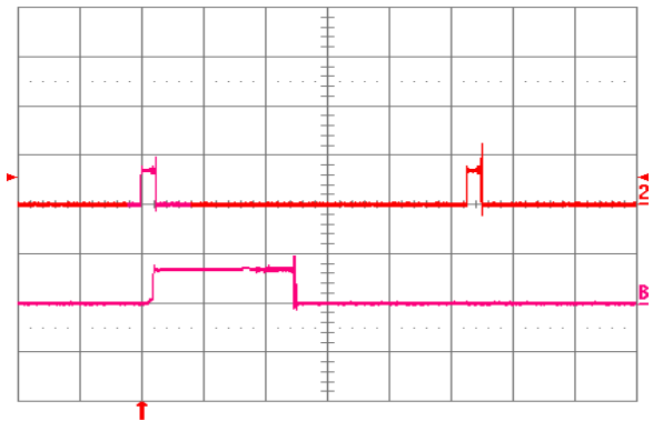
Fig. 6.0V.18: Load current (top trace, 20 A/div., 20 ms/div.) into a 10\text{m}\Omega short circuit during restart, at V_{in} = 24\text{V} . Bottom trace (20 A/div., 2 ms/div.) is an expansion of the on-time portion of the top trace.
