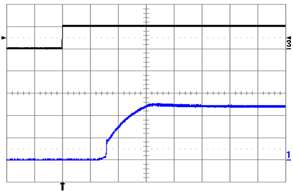
Fig. 1.2V.10: Turn-on transient at full rated load current (resistive) plus 10,000 \mu\text{F} at V_{in} = 24\text{V} , triggered via ON/OFF pin. Top trace: ON/OFF signal (5 V/div.). Bottom trace: output voltage (0.5 V/div.). Time scale: 1 ms/div.
