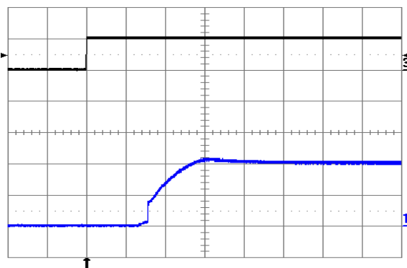
Fig. 1.0V.10: Turn-on transient at full rated load current (resistive) plus 10,000\mu\text{F} at V_{in} = 24\text{V} , triggered via ON/OFF pin. Top trace: ON/OFF signal (5 V/div.). Bottom trace: output voltage (0.5 V/div.). Time scale: 1 ms/div.
