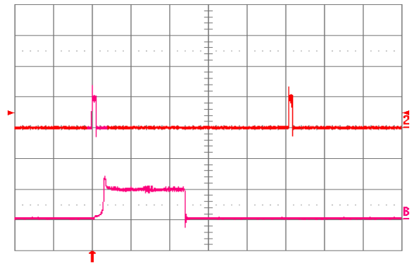
Fig. 2.5V.18: Load current (top trace, 20 A/div., 20 ms/div.) into a 10 \text{m}\Omega short circuit during restart, at V_{in} = 24 \text{ V} . Bottom trace (20 A/div., 1 ms/div.) is an expansion of the on-time portion of the top trace.
