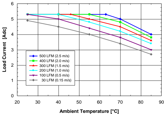
Fig. 8.0V.1: Available load current vs. ambient air temperature and airflow rates for SQ24T/S05080 converter with D height pins mounted vertically with Vin = 24 V, air flowing from pin 3 to pin 1 and maximum FET temperature ≤ 120°C.
