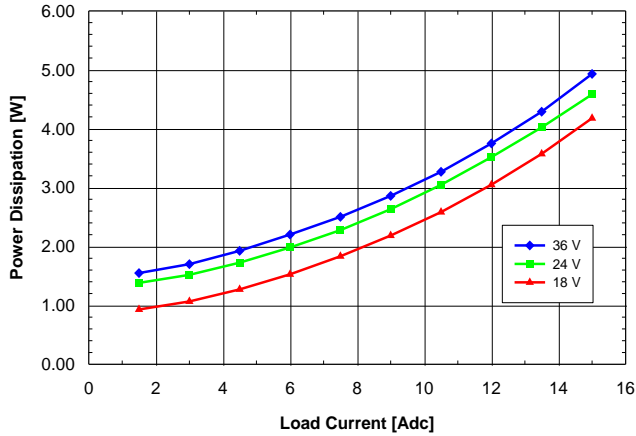
Fig. 1.5V.7: Power dissipation vs. load current and input voltage for SQ24T/S15015 converter mounted vertically with air flowing from pin 3 to pin 1 at a rate of 300 LFM (1.5 m/s) and T_a = 25^\circ\text{C} .
