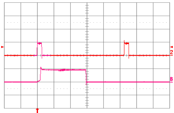
Fig. 1.8V.18: Load current (top trace, 20 A/div., 20 ms/div.) into a 10 m \Omega short circuit during restart, at V_{in} = 24 \text{ V} . Bottom trace (20 A/div., 2 ms/div.) is an expansion of the on-time portion of the top trace.
