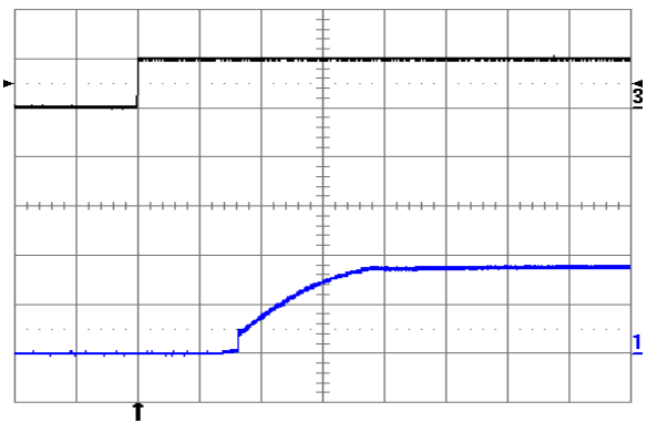
Fig. 1.8V.10: Turn-on transient at full rated load current (resistive) plus 10,000\mu\text{F} at V_{in} = 24\text{V} , triggered via ON/OFF pin. Top trace: ON/OFF signal (5 V/div.). Bottom trace: output voltage (1 V/div.). Time scale: 1 ms/div.
