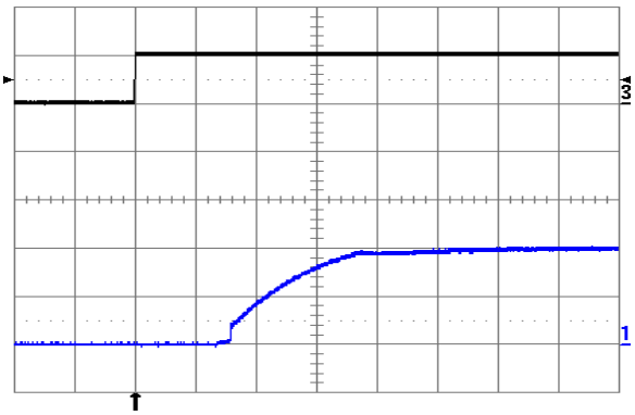
Fig. 2.0V.10: Turn-on transient at full rated load current (resistive) plus 10,000\mu\text{F} at V_{in} = 24\text{V} , triggered via ON/OFF pin. Top trace: ON/OFF signal (5 V/div.). Bottom trace: output voltage (1 V/div.). Time scale: 1 ms/div.
