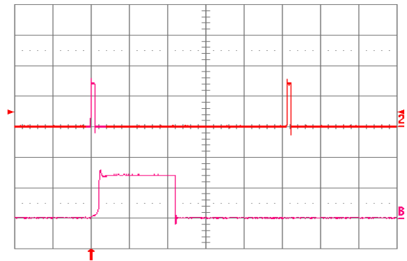
Fig. 5.0V.18: Load current (top trace, 10 A/div., 20 ms/div.) into a 10 \text{m}\Omega short circuit during restart, at V_{in} = 24 \text{ V} . Bottom trace (10 A/div., 1 ms/div.) is an expansion of the on-time portion of the top trace.
