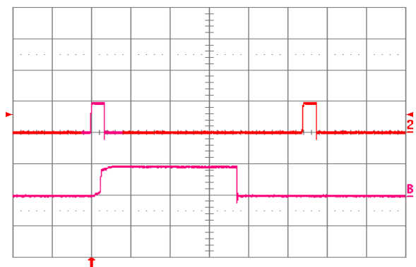
Fig. 1.0V.18: Load current (top trace, 20 A/div., 20 ms/div.) into a 10 \text{m}\Omega short circuit during restart, at V_{in} = 24 \text{ V} . Bottom trace (20 A/div., 2 ms/div.) is an expansion of the on-time portion of the top trace.
