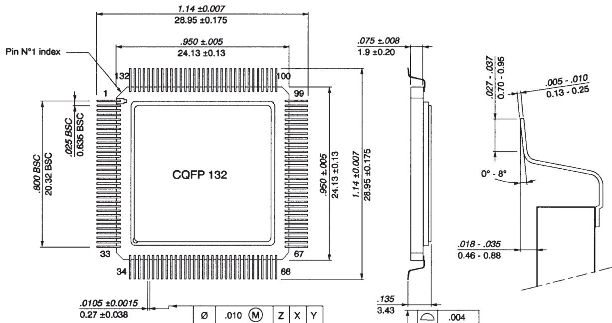
Figure 12-2. 132 Pins - Ceramic Quad Flat Pack
