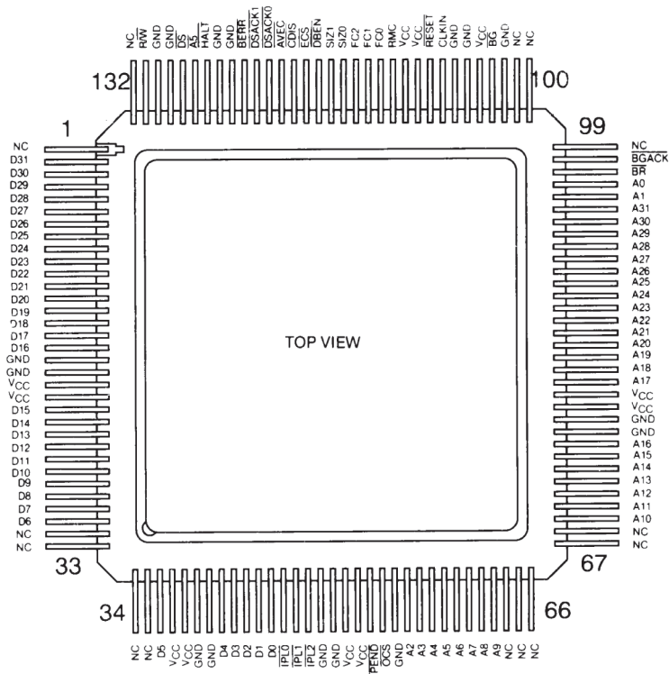
Figure 1-3. CQFP Terminal Designation
