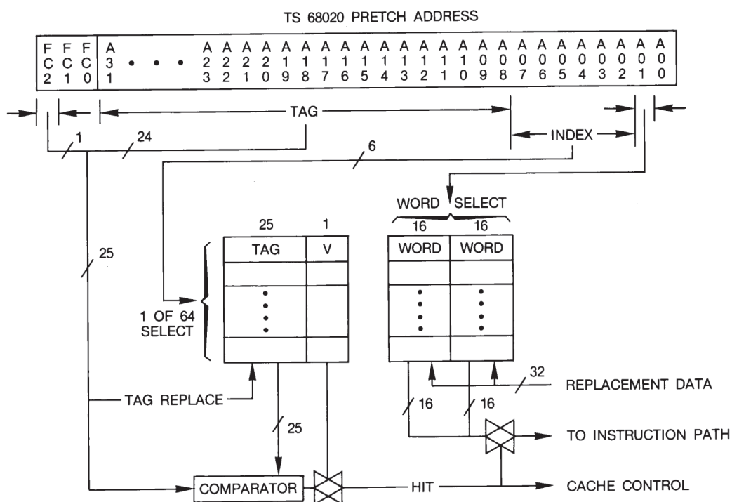
Figure 9-4. TS68020 On-chip Cache Organization
