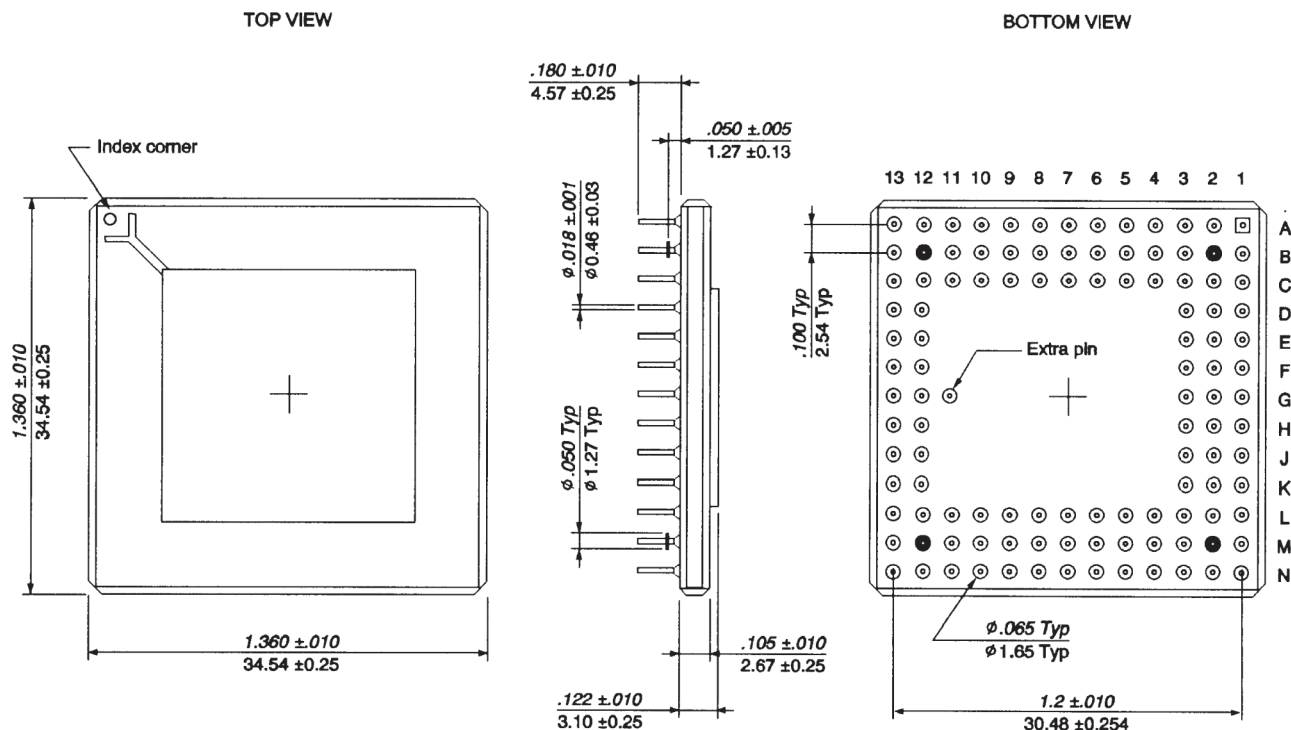
Figure 12-1. 114-lead - Ceramic Pin Grid Array
