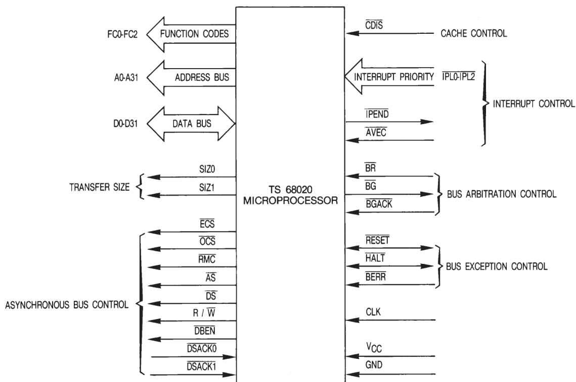
Figure 1-4. Functional Signal Groups
