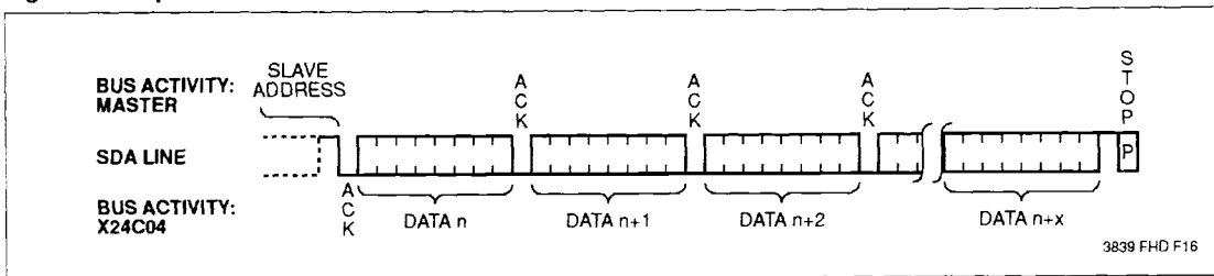
Figure 9. Sequential Read
