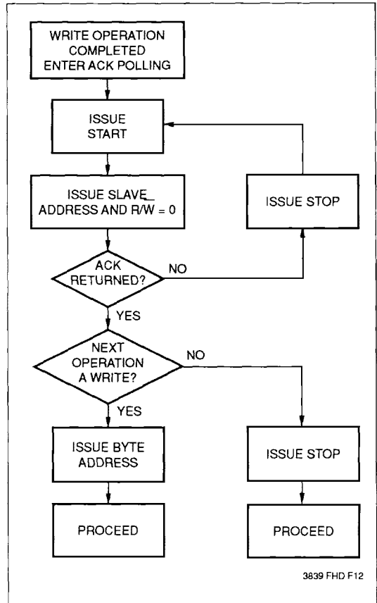
Flow 1. ACK Polling Sequence
