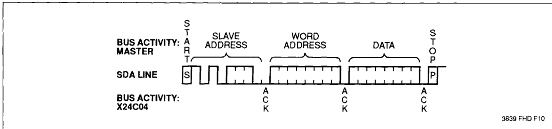
Figure 5. Byte Write
