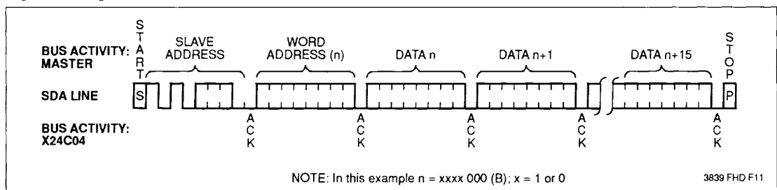
Figure 6. Page Write
