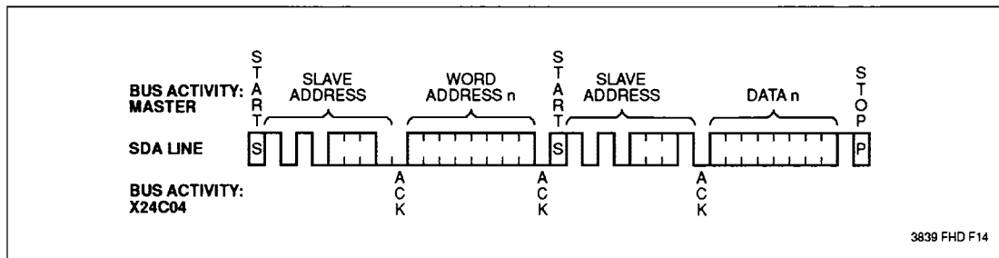
Figure 8. Random Read
