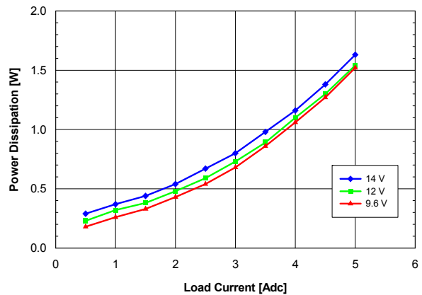
Fig. 1.0V.4: Power Loss vs. load current and input voltage for V_{out} = 1.0V converter mounted vertically with air flowing from pin 5 to pin 1 at a rate of 200 LFM (1 m/s) and T_a = 25^{\circ} .
