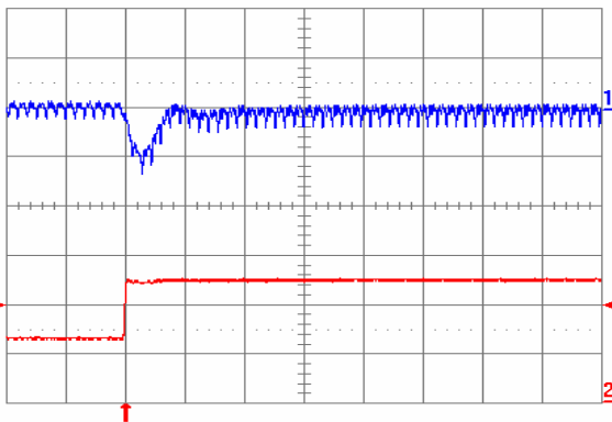
Fig. 2.0V.7: Output voltage response for V_{out} = 2.0V to a positive load current step change from 2.5A to 5A with a slew rate of 5A/\mu s at V_{in} = 12V . Top trace: output voltage (100mV/div); Bottom trace: load current (2A/div). C_o = 47\mu F ceramic. Time scale: 20 \mu s /div.
