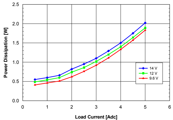
Fig. 2.5V.4: Power Loss vs. load current and input voltage for V_{out} = 2.5V converter mounted vertically with air flowing from pin 5 to pin 1 at a rate of 200 LFM (1 m/s) and T_a = 25^{\circ} .
