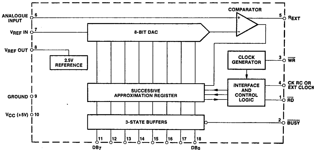
Fig.1 System diagram
